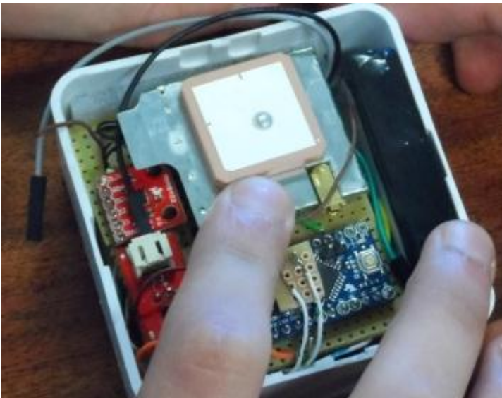
Figure 2. Prototype of the Pet Tracker II
